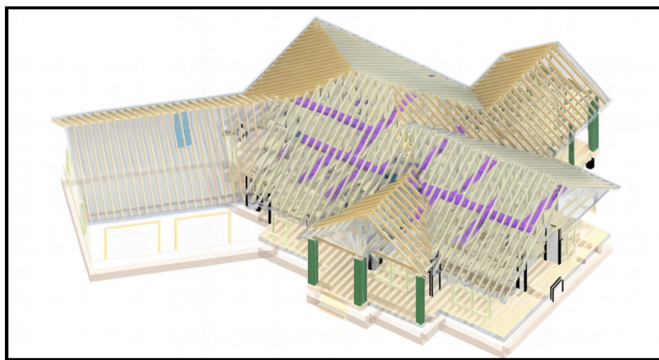
STRUCTURE BIM
